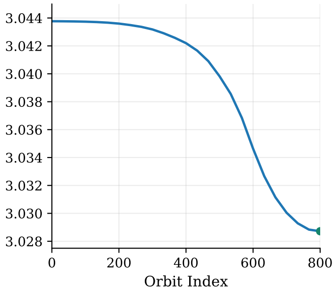
Jacobi Constant
