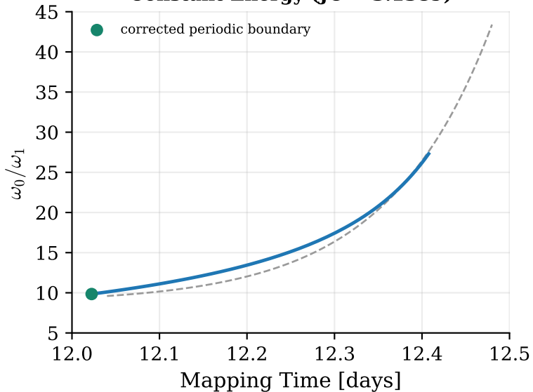
Quasi-Halo Family Constant Energy (JC = 3.1389)
