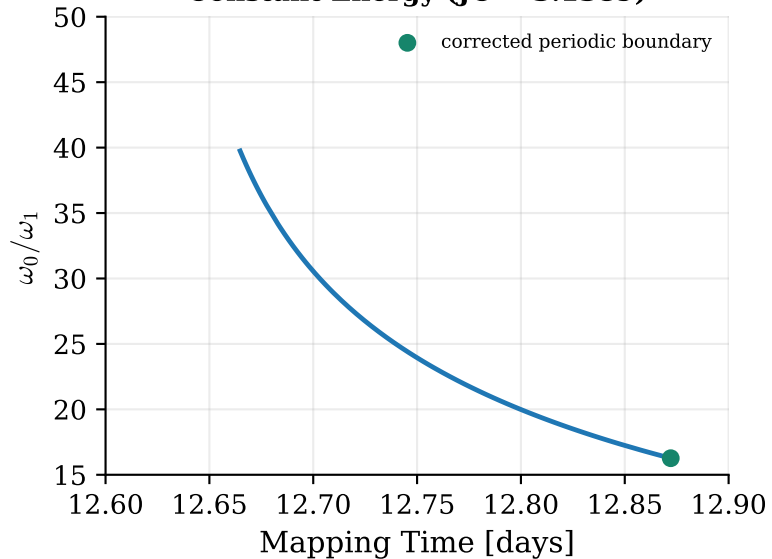
Quasi-Vertical Family Constant Energy (JC = 3.1389)
