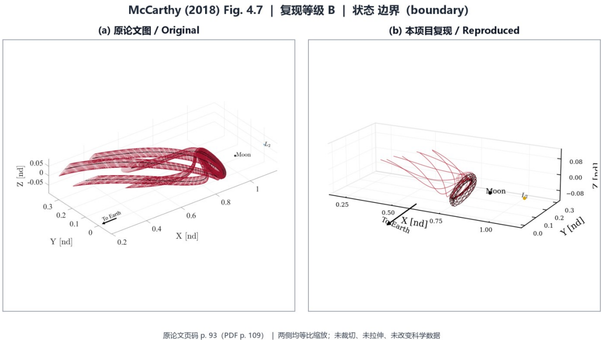
图 39 McCarthy 原文结果与本文复现结果对照（原论文 Fig. 4.7）：（a）原论文图；（b）本项目复现图 Fig. 39 Comparison between the original result of McCarthy (Fig. 4.7) and the result reproduced in this work: (a) original; (b) reproduced
