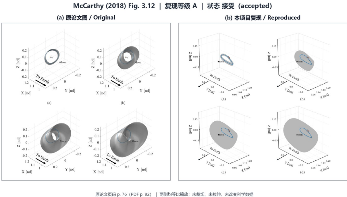
图 27 McCarthy 原文结果与本文复现结果对照（原论文 Fig. 3.12）：（a）原论文图；（b）本项目复现图 Fig. 27 Comparison between the original result of McCarthy (Fig. 3.12) and the result reproduced in this work: (a) original; (b) reproduced
