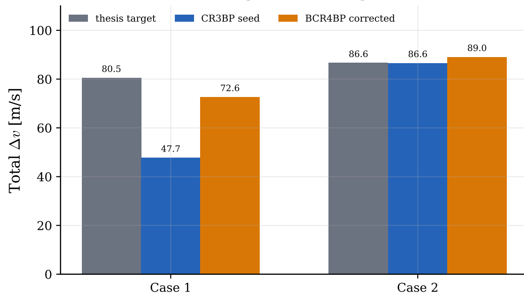
(c) Two-impulse total \Delta v comparison
