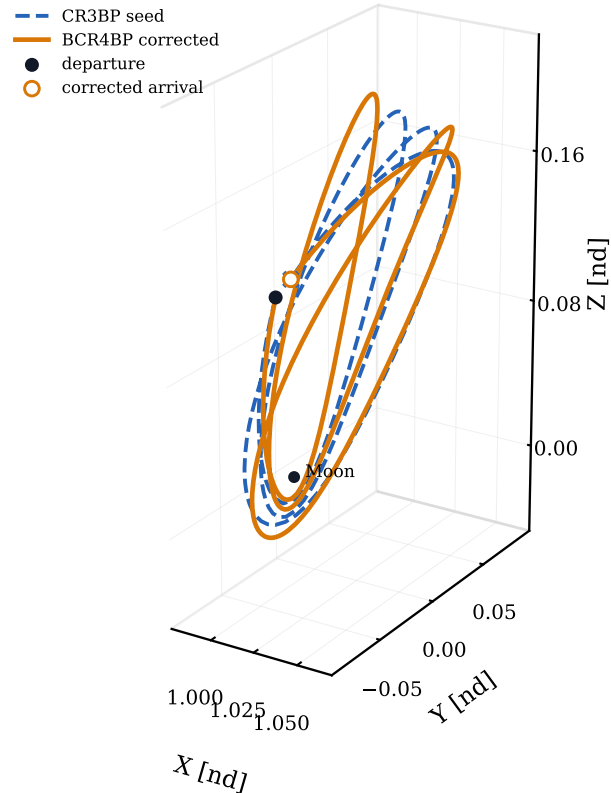
(a) Case 1: 23.0 d | numerical PASS
