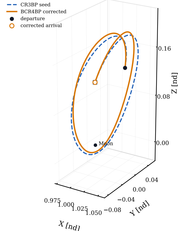
(b) Case 2: 12.4 d | numerical PASS
