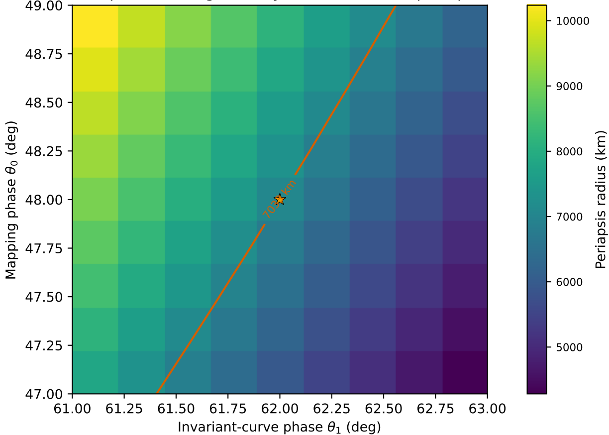
Accepted active-geometry stable-manifold periapsis
