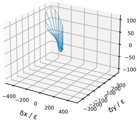
b Partial real Schur
