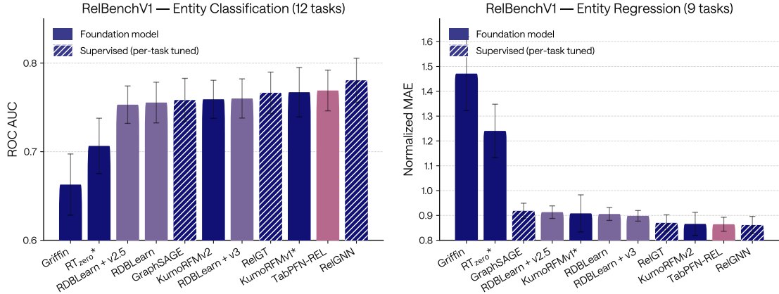
Figure 21. TabPFN-3 tops performance on RelBenchV1 among foundation models. Following Hudovernik et al. [58], we report the mean ROC AUC for entity classification and MAE scores for entity regression normalized by LightGBM’s MAE. RelGNN [59] achieves SOTA performance on both tasks, followed by TabPFN-REL, which sets a new SOTA for foundation models. Methods marked with * in their name (KumoRFMv1, RT zero ) indicate methods that are likely following a different evaluation protocol than the one outlined in RelBench, which overestimates model performance.
