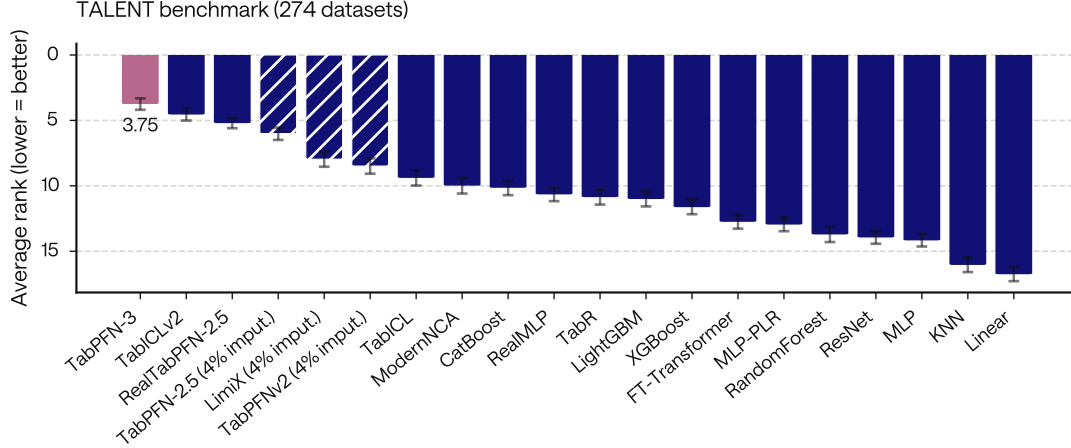
Figure 13. Average rank on the TALENT benchmark, using the TabICLv2 evaluation protocol from Qu et al. [30] (274 datasets). The original 300-dataset TALENT [38] minus the 26 development datasets used for TabPFN-2 / TabICLv2 development removed in the TabICLv2 paper), spanning regression, binary and multiclass classification. Bars show mean rank (lower is better); error bars are 95% bootstrap confidence intervals over datasets (see appendix E.3). Methods tagged ( N imputed , X% ) failed on some datasets and have that fraction of their score cells filled with K-nearest-neighbour values.
