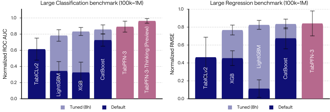
Figure 15. TabPFN-3 achieves state-of-the-art performance on the large-rows benchmark (up to 1M training rows and 200 features, 13 datasets) , outperforming both default and 8-hour-tuned gradient-boosted tree baselines as well as TabICLv2 in a single forward pass. (a) Classification (9 datasets). (b) Regression (4 datasets) use temporal splits. Normalized scores are higher-is-better; see Section F.1 for the normalization procedure and Appendix F.2 for critical difference diagrams.
