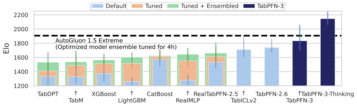
Figure 1. Performance on the TabArena benchmark [1], largest data subset (10k-100k samples). TabPFN-3 outperforms any other model in a forward pass. TabPFN-3-Plus (Thinking) is dramatically better yet, outperforming AutoGluon 1.5 extreme [2], a complex ensemble of models tuned for 4 hours, while being 10x faster.
