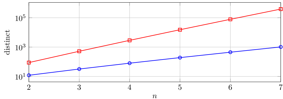
Search Depth
