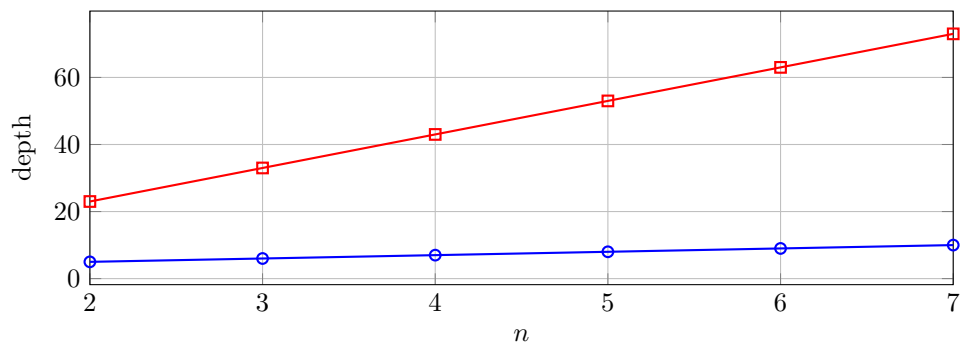
Search Depth
