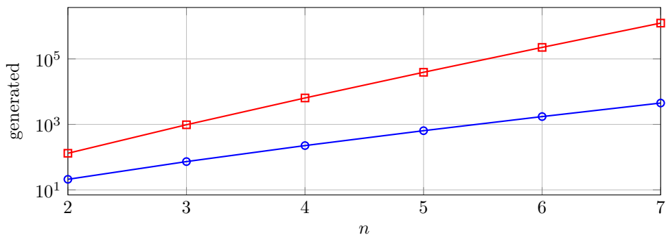
Distinct States
