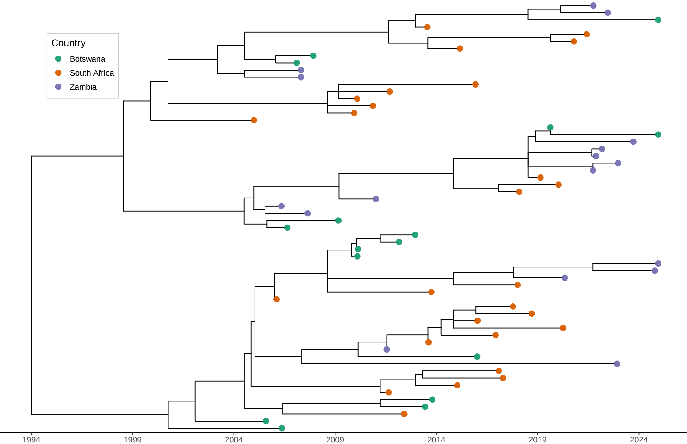
Dataset B – SIMULATED epidemic
