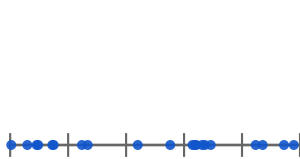
1 feature: 5 cells
