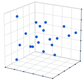
3 features: 125 cells
