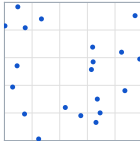
2 features: 25 cells
