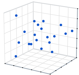
3 features: 125 cells
