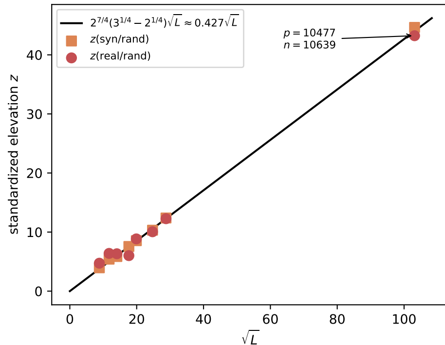
(B) Growth law: elevation \propto \sqrt{L} toward the 3/2 ceiling
