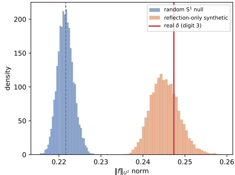
(A) Null distributions, L = 828 (increment-shuffle null \equiv random, z \approx 0 )
