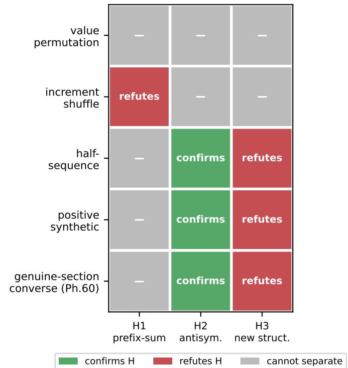
(C) Hypothesis \times control matrix (permutation alone cannot separate)
