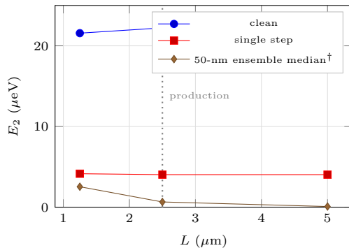
(b) length convergence ( dx = 5\ \text{nm} )
