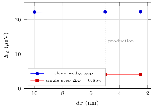
(a) lattice-spacing convergence ( L = 2.5\ \mu\text{m} )
