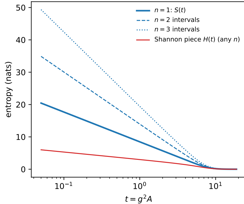
(b) SU(3): S_n = H + 2n\langle \ln d \rangle , all decreasing
