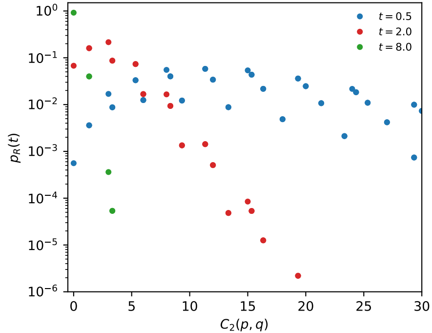
(a) SU(3) flux distribution p_R \propto d_R^2 e^{-tC_2/2}
