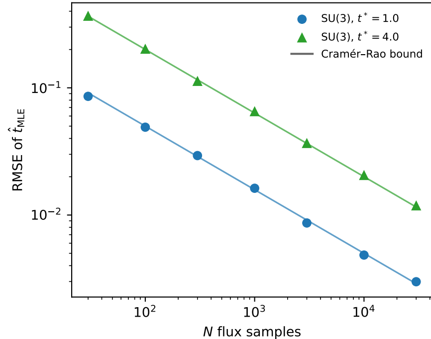
(c) SU(3) reconstruction vs CRB
