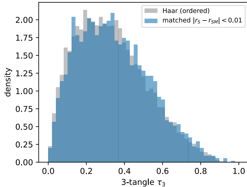
(b) Matching manifold is generic
