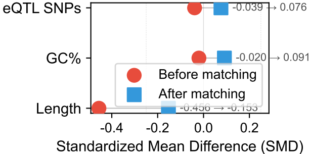
Figure 4. Covariate Balance (Love Plot)
