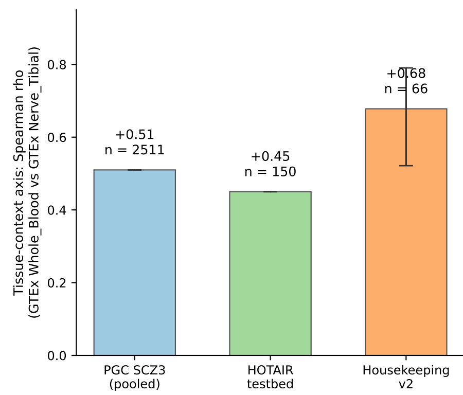
(c) Tissue-context axis across gene sets
