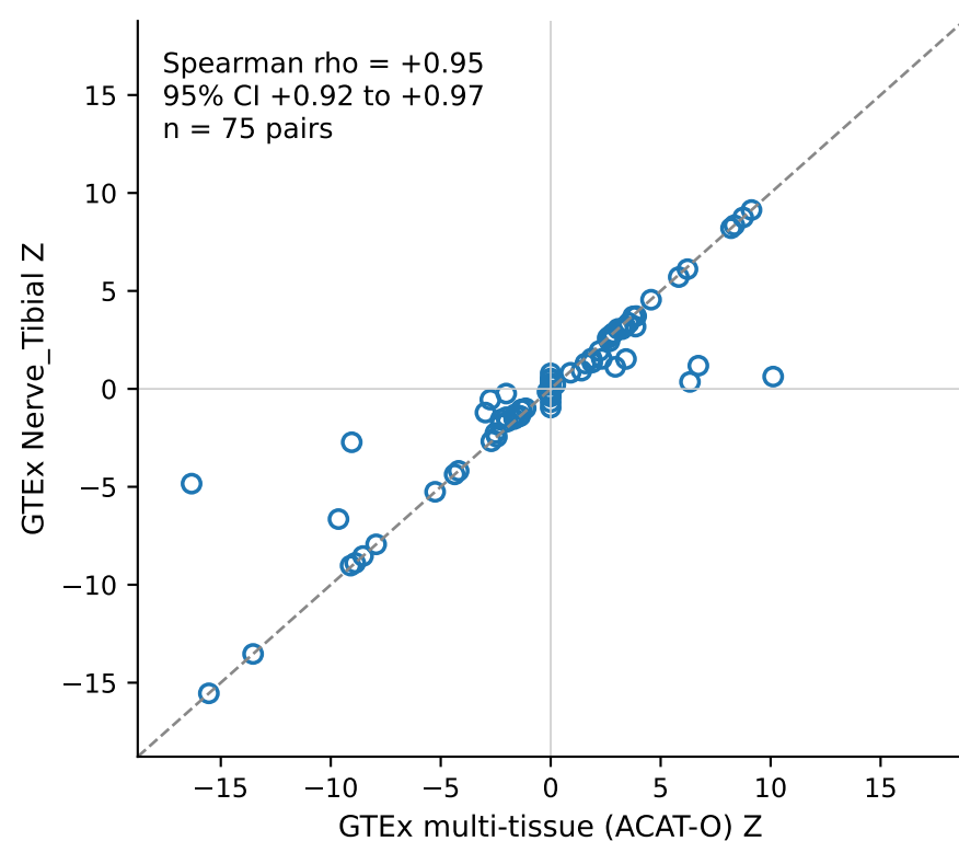
(a) Housekeeping true-negative control (v2)
