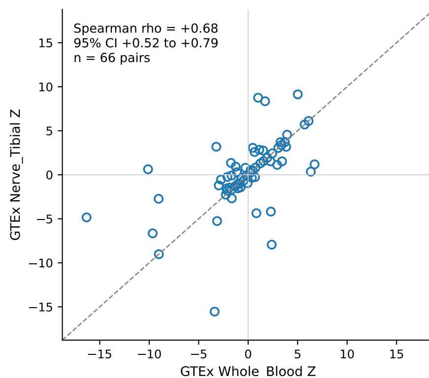
(b) Housekeeping true-negative control (v2)
