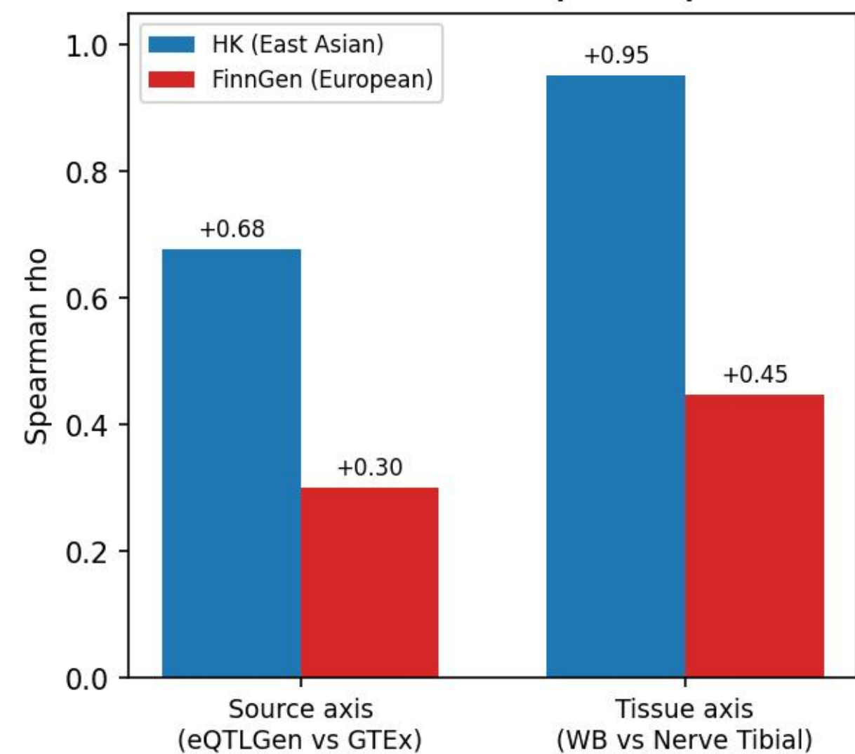
C. Decomposition rho: HK vs FinnGen (Pooled)
