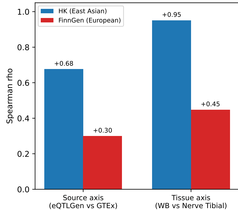
C. Decomposition rho: HK vs FinnGen (Pooled)
