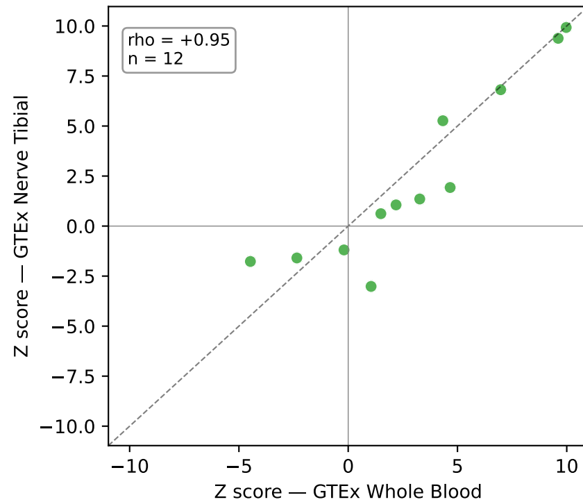
B. Tissue axis (HK) Whole Blood vs Nerve Tibial
