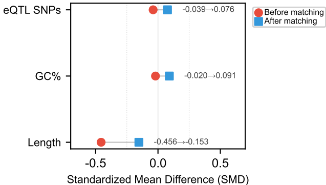
Figure 4. Covariate Balance (Love Plot)
