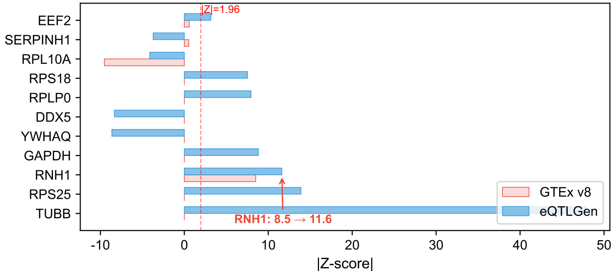
Figure 2. Core Gene |Z-score|: GTEx vs eQTLGen (DR)
