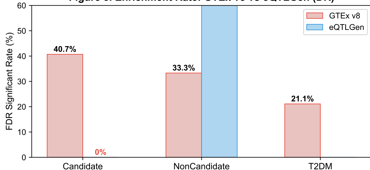
Figure 3. Enrichment Rate: GTEx v8 vs eQTLGen (DR)
