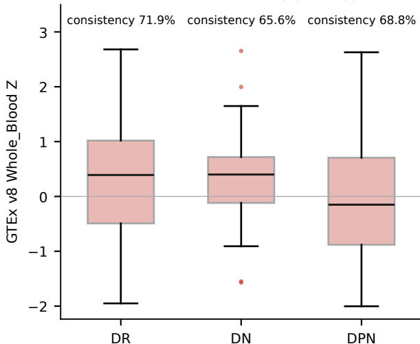
(b) GTEx Z distribution by phenotype
