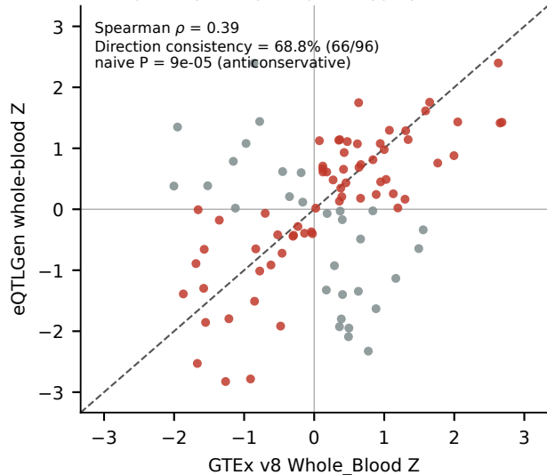
(a) 96 primary-arm gene-phenotype pairs (official Z)
