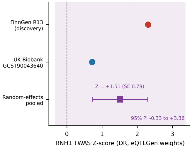
(b) Cross-cohort replication
