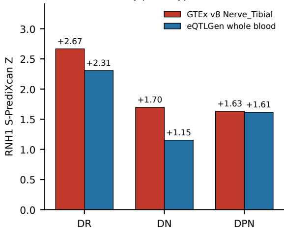
(a) RNH1 by phenotype (official Z)
