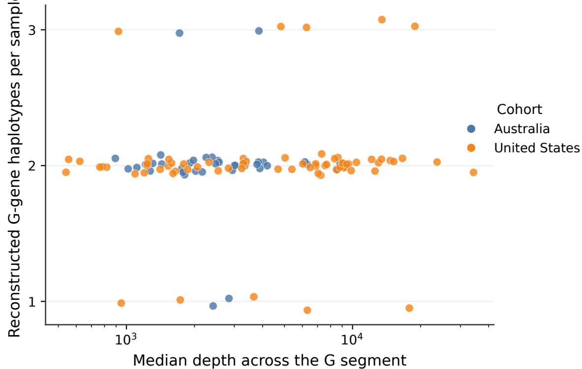
Depth and haplotype number
