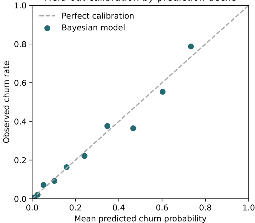
Held-out calibration by prediction decile
