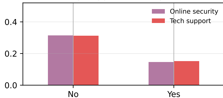
Churn by support/security features
