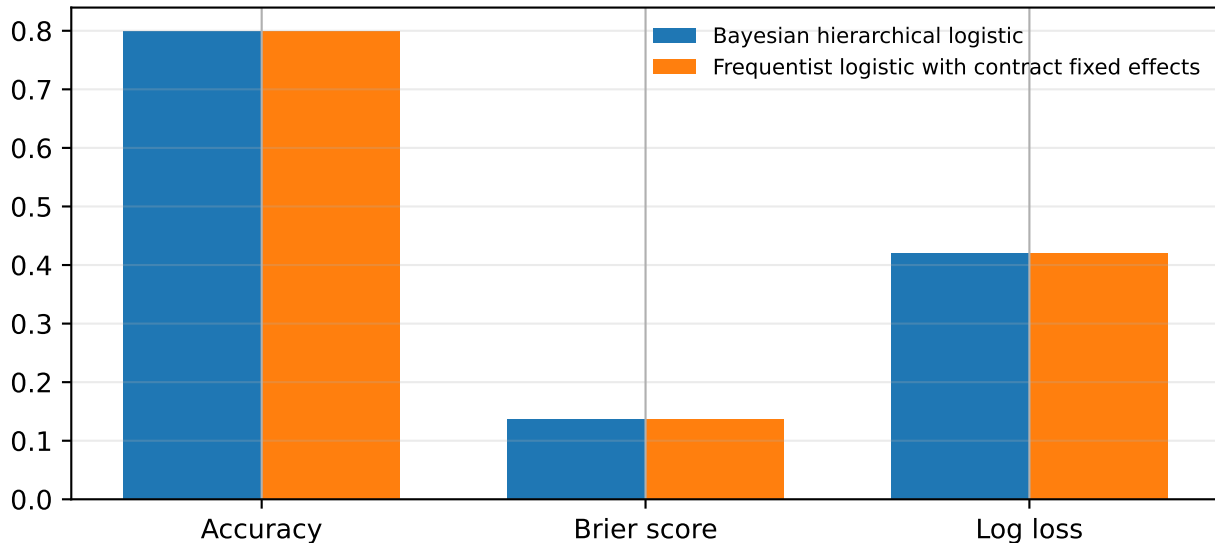
In-sample predictive comparison
