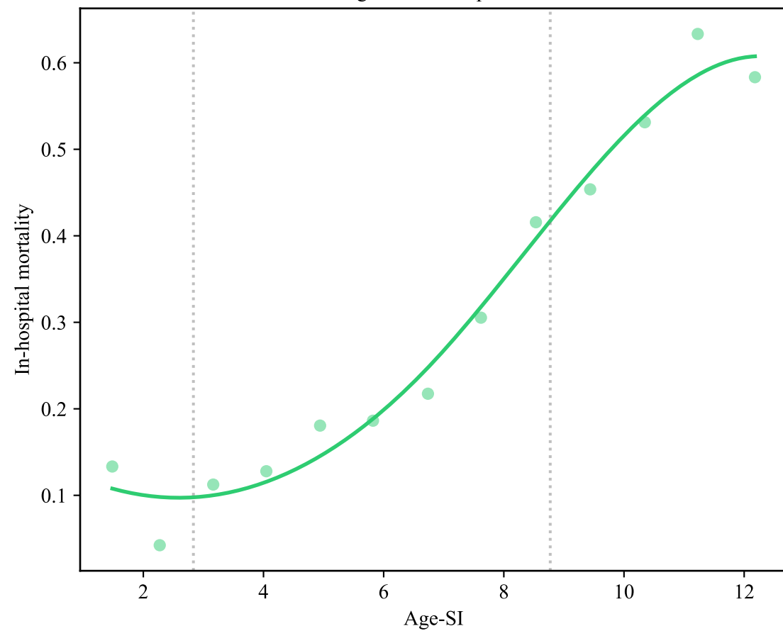
Age-SI dose-response
