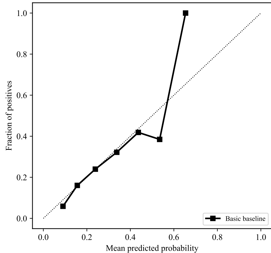
Basic baseline
