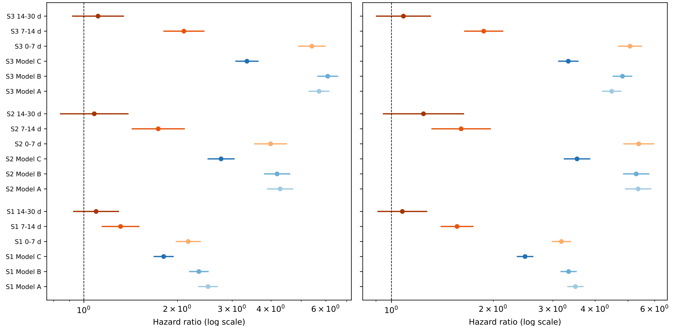
MIMIC-IV: stage HRs (TV Cox)
