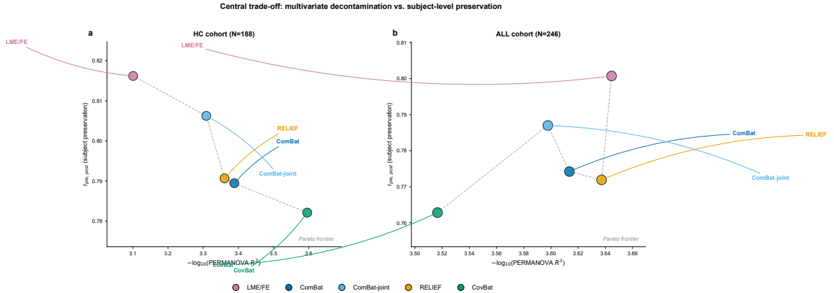
Figure 3: Pareto frontier showing the trade-off between multivariate vendor-effect removal (PERMANOVA R^2 , permutational multivariate analysis of variance) and subject-level preservation (Pearson correlation r_{\text{pre,post}} between pre- and post-harmonisation biomarker vectors). (a) Healthy control cohort ( N = 188 ); (b) pathology-inclusive cohort ( N = 246 ). A monotone frontier is present in the HC cohort; in the pathology-inclusive cohort the ordering is non-monotone (Section 3.5). Each point represents one harmonisation method. Lower right indicates maximal vendor-effect removal; upper left indicates maximal subject-level preservation.
