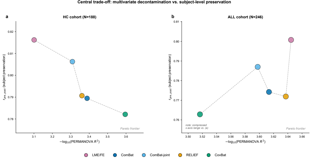
Figure 3: Pareto frontier showing the trade-off between multivariate vendor-effect removal (PERMANOVA R^2 , permutational multivariate analysis of variance) and subject-level preservation (Pearson correlation r_{pre,post} between pre- and post-harmonisation biomarker vectors). (a) Healthy control cohort ( N = 188 ); (b) pathology-inclusive cohort ( N = 246 ). A monotone frontier is present in the HC cohort; in the pathology-inclusive cohort the ordering is non-monotone (Section 3.5). Each point represents one harmonisation method. Lower right indicates maximal vendor-effect removal; upper left indicates maximal subject-level preservation. The x -axis range in (b) is compressed relative to (a) (flagged in the panel), so the apparent spread of methods on this axis should not be compared directly between panels.
