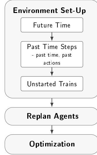
Fig. 2: High-level overview of Secondary Encoding.
