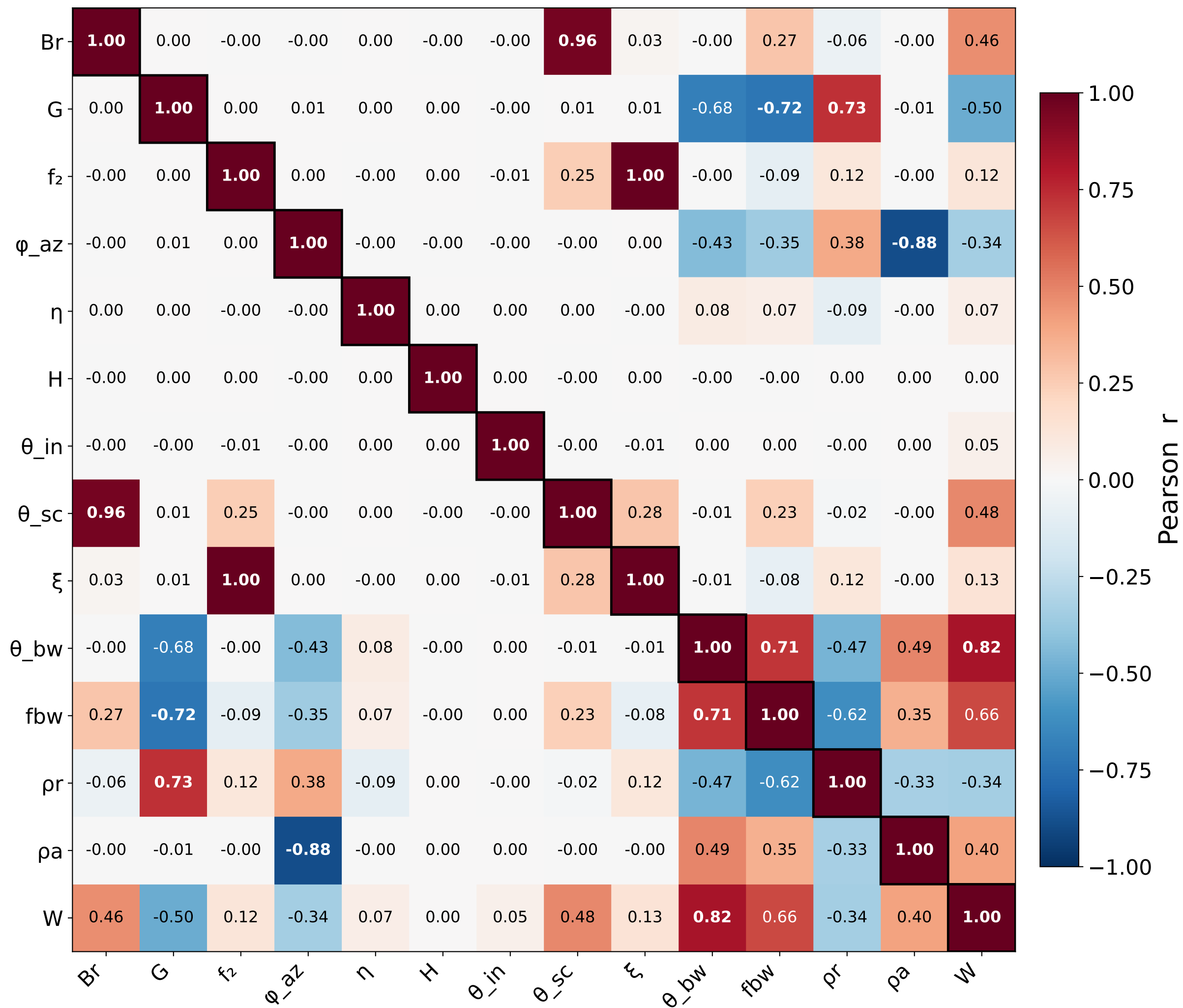
Pearson Correlation Matrix (N = 100000 valid samples; G \in [25, 40] dB, f_2 \in [25, 60] GHz)
