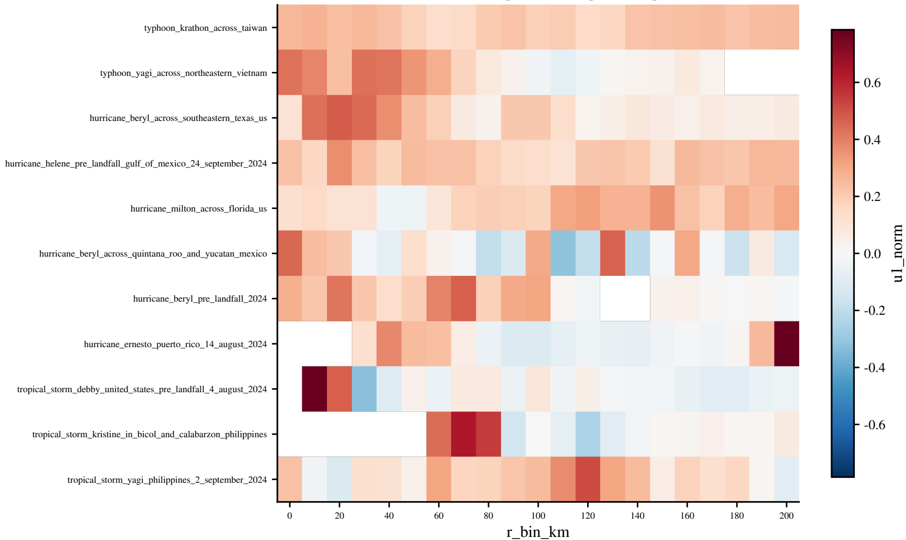
f(r)=u_1(r) (normalized) heatmap; value_col= \phi _overlap, r_max=200km
