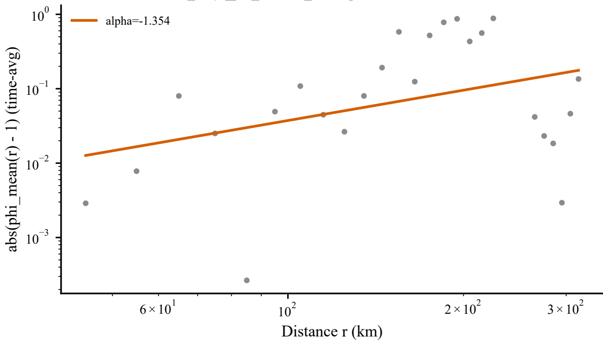
hurricane_beryl_pre_landfall_2024: power-law fit, t in [24.0,72.0]h
