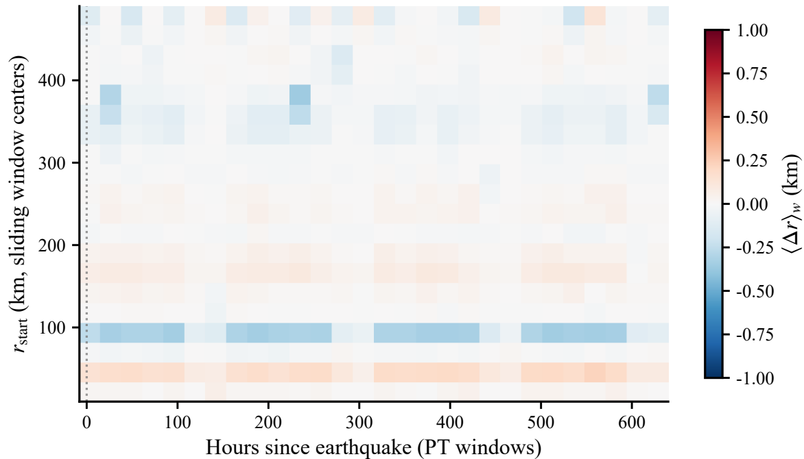
Weighted mean radial displacement \langle \Delta r \rangle_w(r, t)
