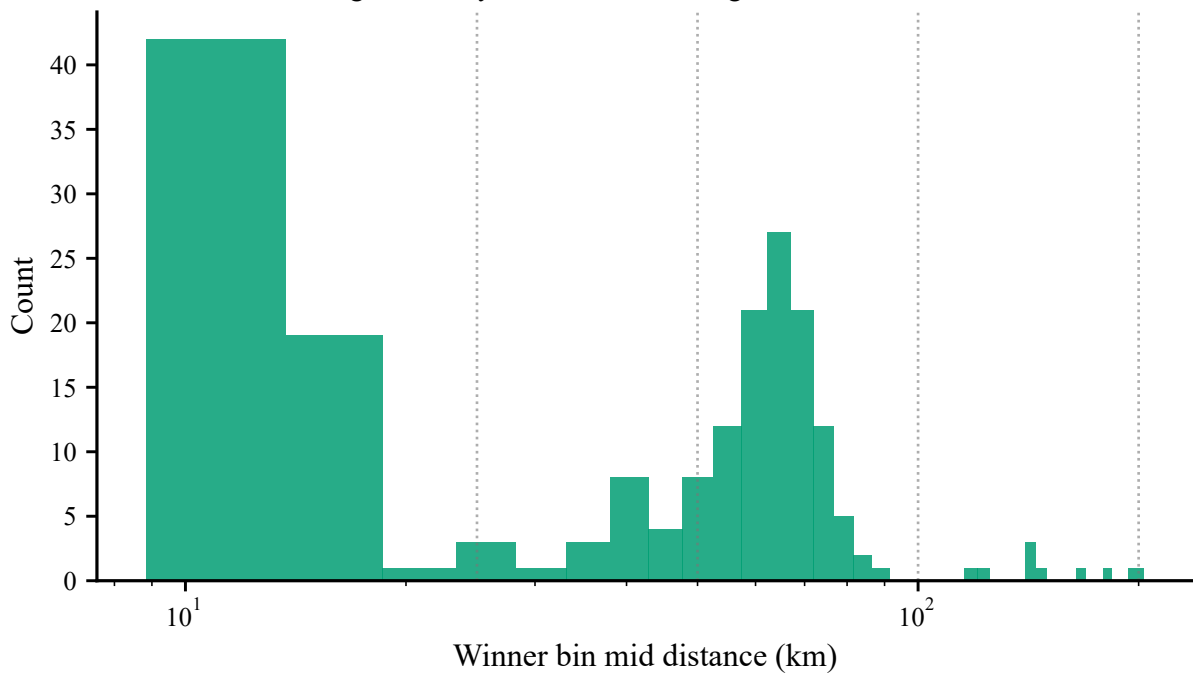
Binning sensitivity: which distance range minimizes median \tau_i ?
