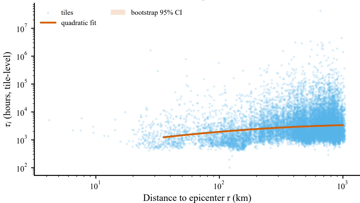
Continuous \tau(r) from tile-level exponential fits (08:00 windows)
