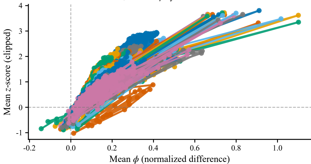
z -score vs \phi by distance bin
