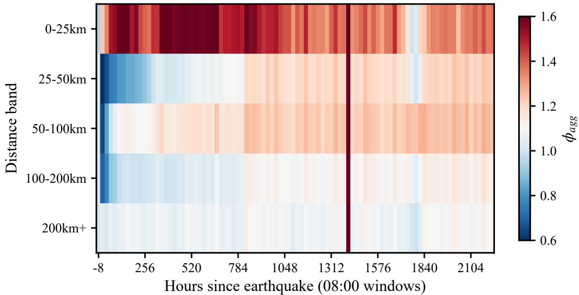
\phi(r, t) heatmap
