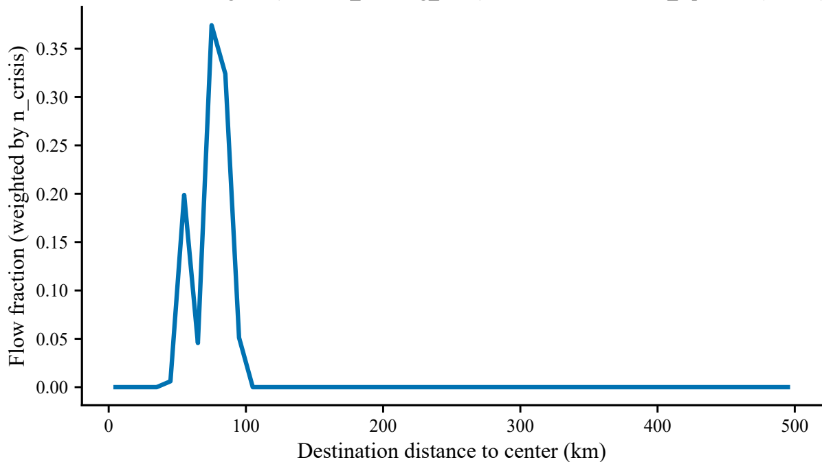
Destination distance histogram (moldova_flooding_2024)\nstart=50-100km, cos_alpha < 0 (inward), t
