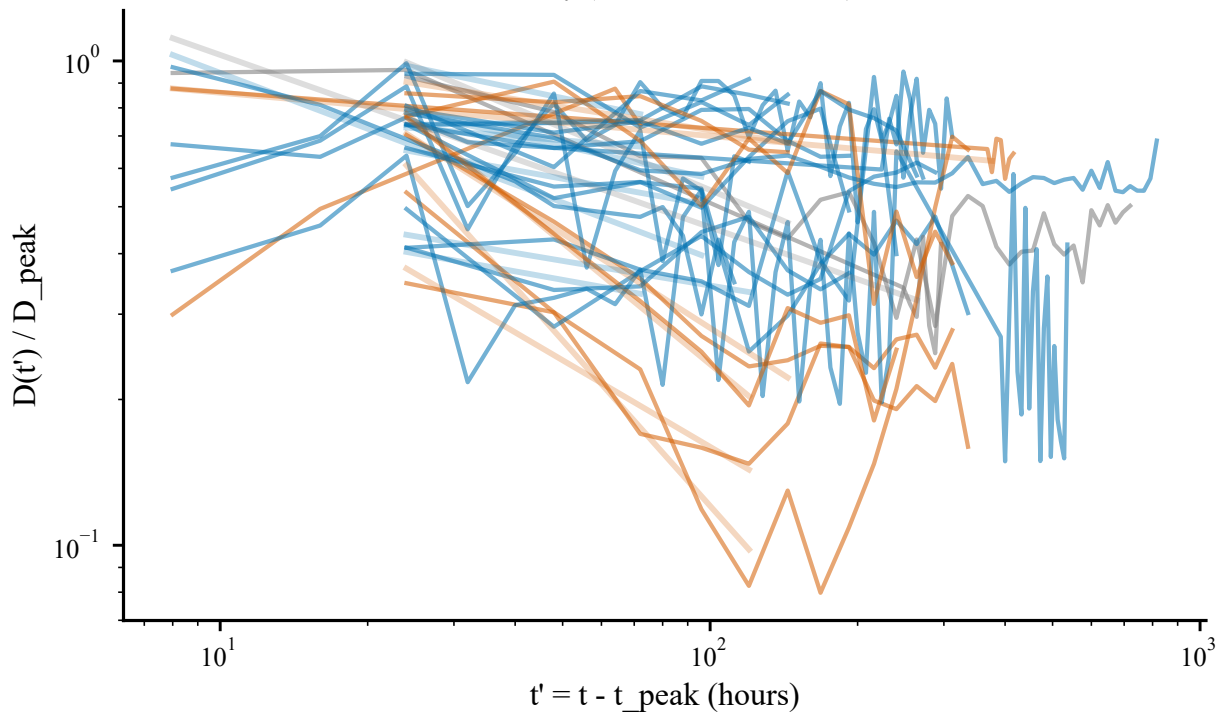
Dt decay (all events, r \leq 200\text{km} )
