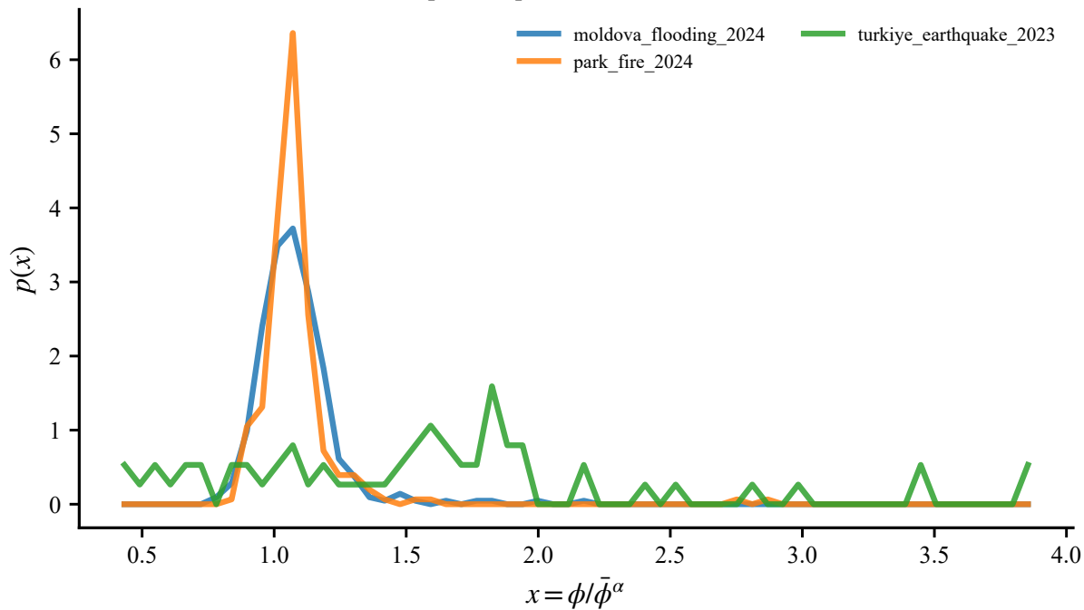
Collapse at \alpha^*=0 for band 0-25km
