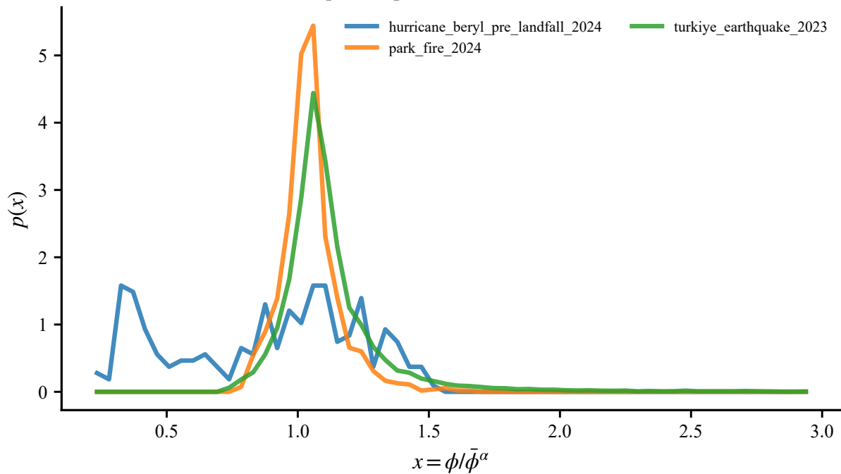
Collapse at \alpha^*=0.1 for band 200km+
