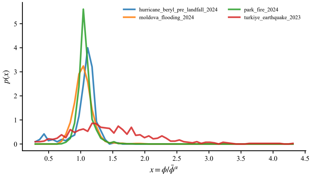
Collapse at \alpha^*=0.05 for band 50-100km
