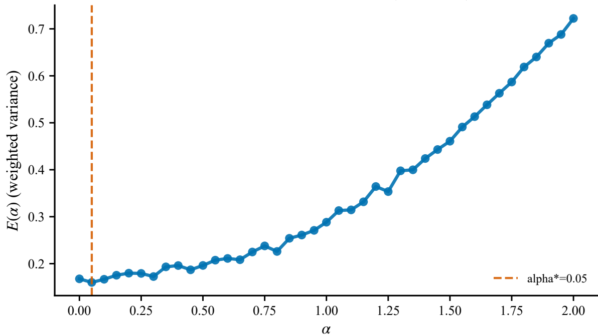
Residual scan for band 100-200km (scale=mean)
