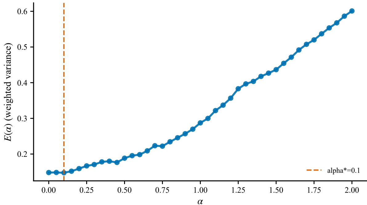
Residual scan for band 200km+ (scale=mean)
